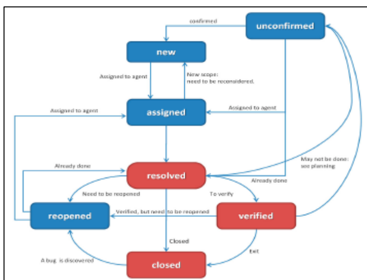
Figure 3: Example of application at instance level
