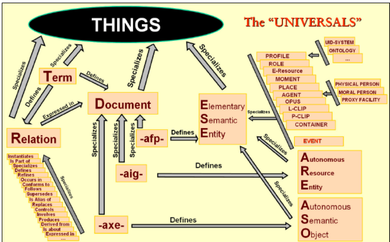
Figure 2: <AXIS-Core classes>
